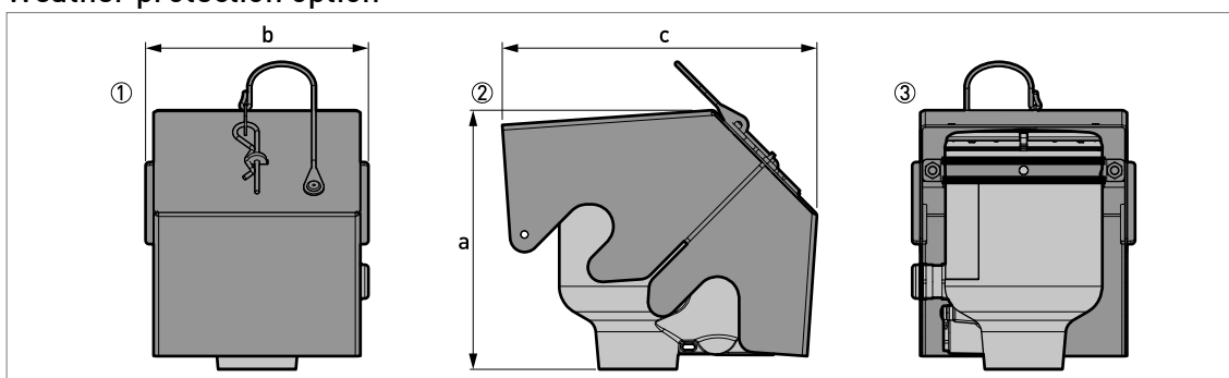
Figure 2-15: Weather protection option
