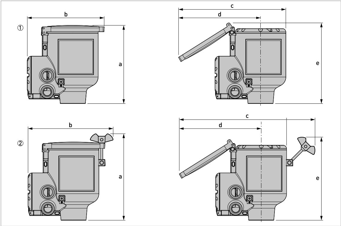
Figure 2-9: Stainless-steel cover options ① Signal converter housing with stainless-steel cover - without locking system ② Signal converter housing with stainless-steel cover - with locking system
