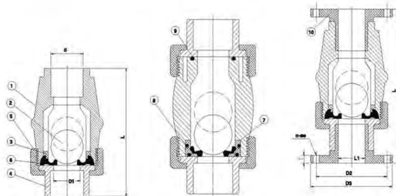
FLANGED 15A(1/2'')-250A(10'')
