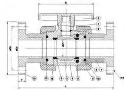
FLANGE TYPE
