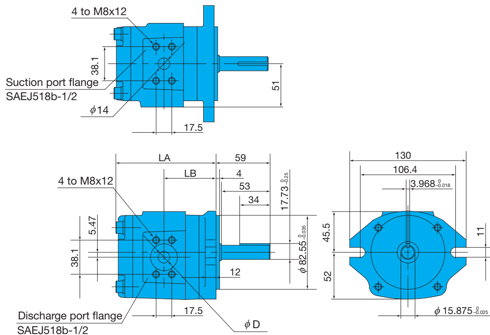
IPH-2B-*-11 (Flange Mounting, Clockwise Rotation)
