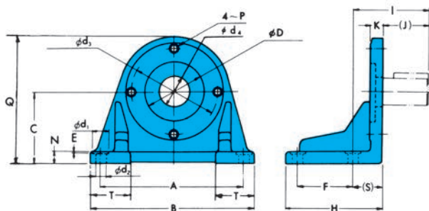
SAE-2BOLT-MOUNTING
