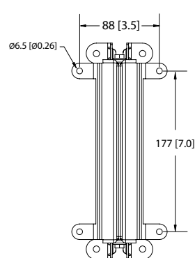
Wall-Mount Section
